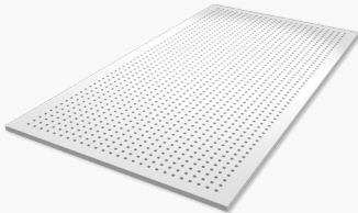
1200mm x 2400mm Gypsum Board Q3, 11.9% 280 x 136 Holes
