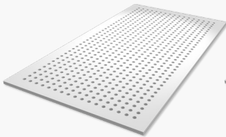
1200mm x 2400mm Gypsum Board R12, 16.4% 45 x 93 Holes
