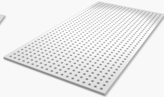
Borderless 1175mm x 2400mm Gypsum Board R12, 18.1% 47 x 96 Holes
