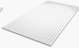
Borderless 1149mm x 2365mm Gypsum Board R6, 11.1% 72 X 148 Holes
