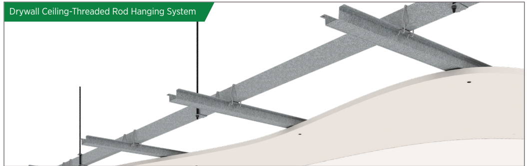
Drywall Ceiling-L Angle Hanging System
